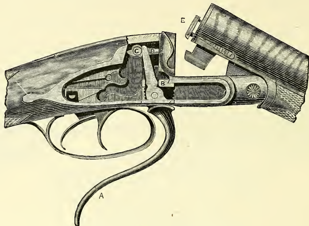
Mechanism of Murcott's Hammerless Gun.
